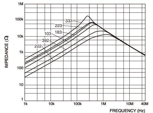
Impedance Characteristics
